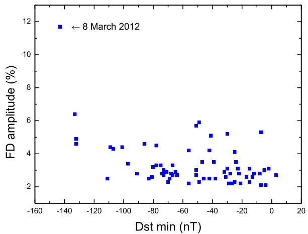
Figure 6 FD amplitudes (%) versus the D_{st} min (nT) values associated with every event. The event of 8 March 2012 is exceptional.
