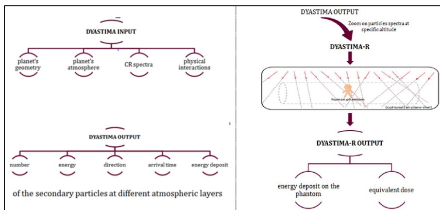
Fig. 1. Block diagram of the software DYASTIMA/DYASTIMA-R
