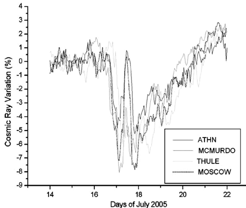
Fig. 4. Cosmic ray variations from 14 to 22 July 2005 from various stations: Athens, McMurdo, Thule and Moscow.
