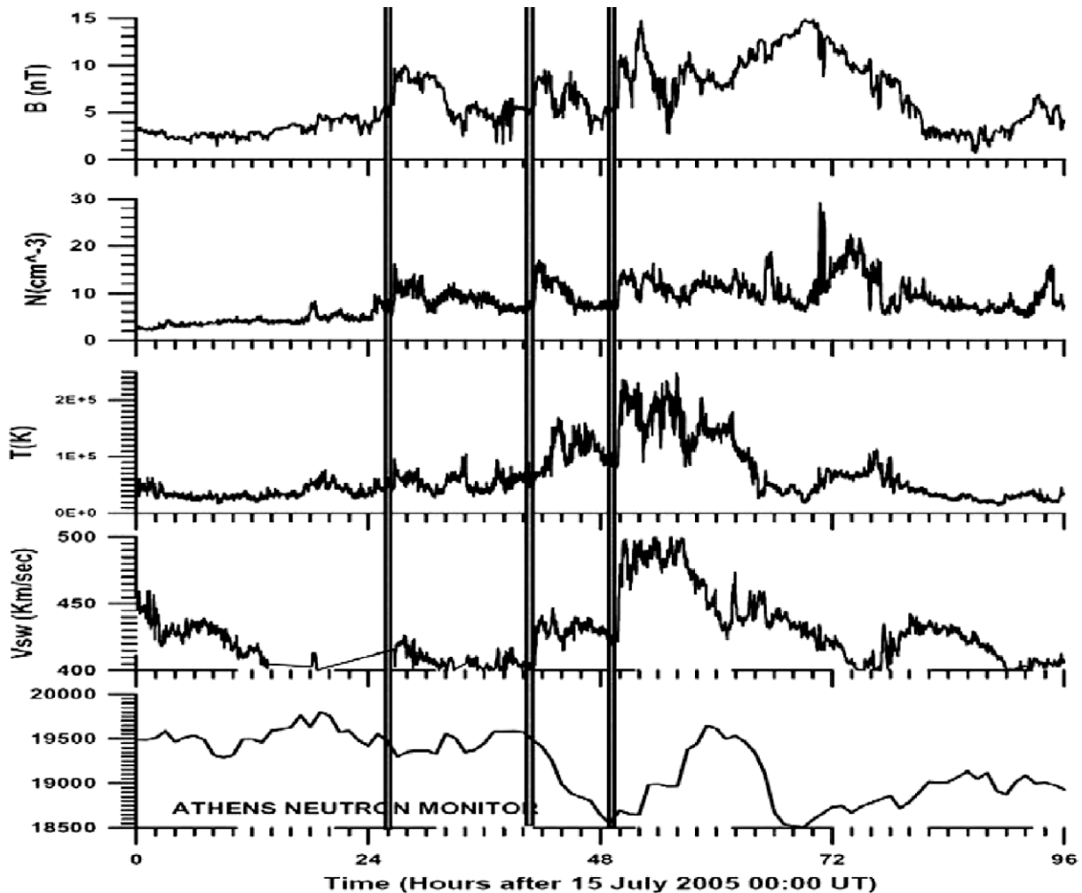
Fig. 3. Solar wind parameters from OMNI; top to bottom: total magnetic field strength, proton density, proton temperature and solar wind speed. Three weak shocks are marked (cf. discussion in text). Bottom: the ANMODAP plot of the irregular Forbush decrease, interrupted by a sudden enhancement.
