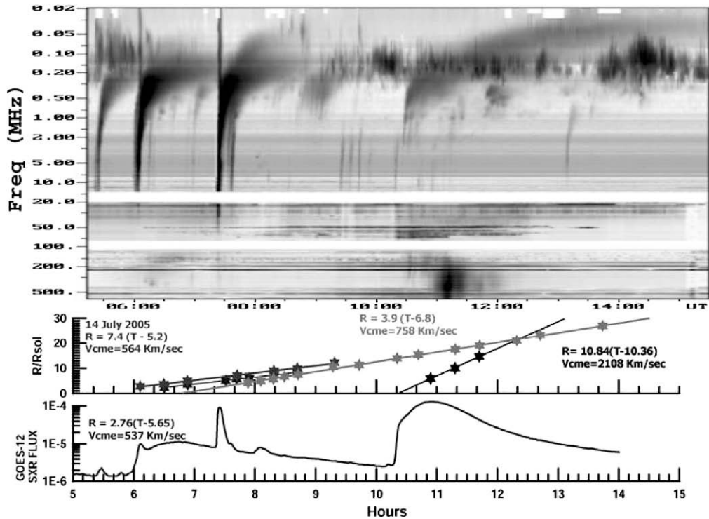
Fig. 2. Top: Composite ARTEMIS-IV/WIND Dynamic Spectrum of the 14 July 2005 event: type III groups extending into the WAVES range; a faint continuum, 06:00–06:30 UT, and a type IV burst, 10:20–12:20 UT. Middle: height time plot of the fast CME overtaking the slow ones. Bottom: the GOES SXR light curve.
